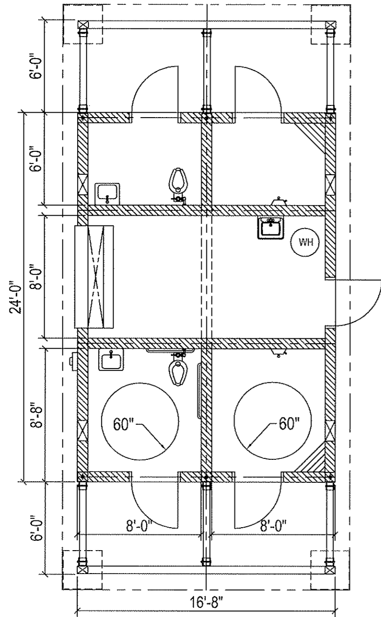
FLOOR PLAN
