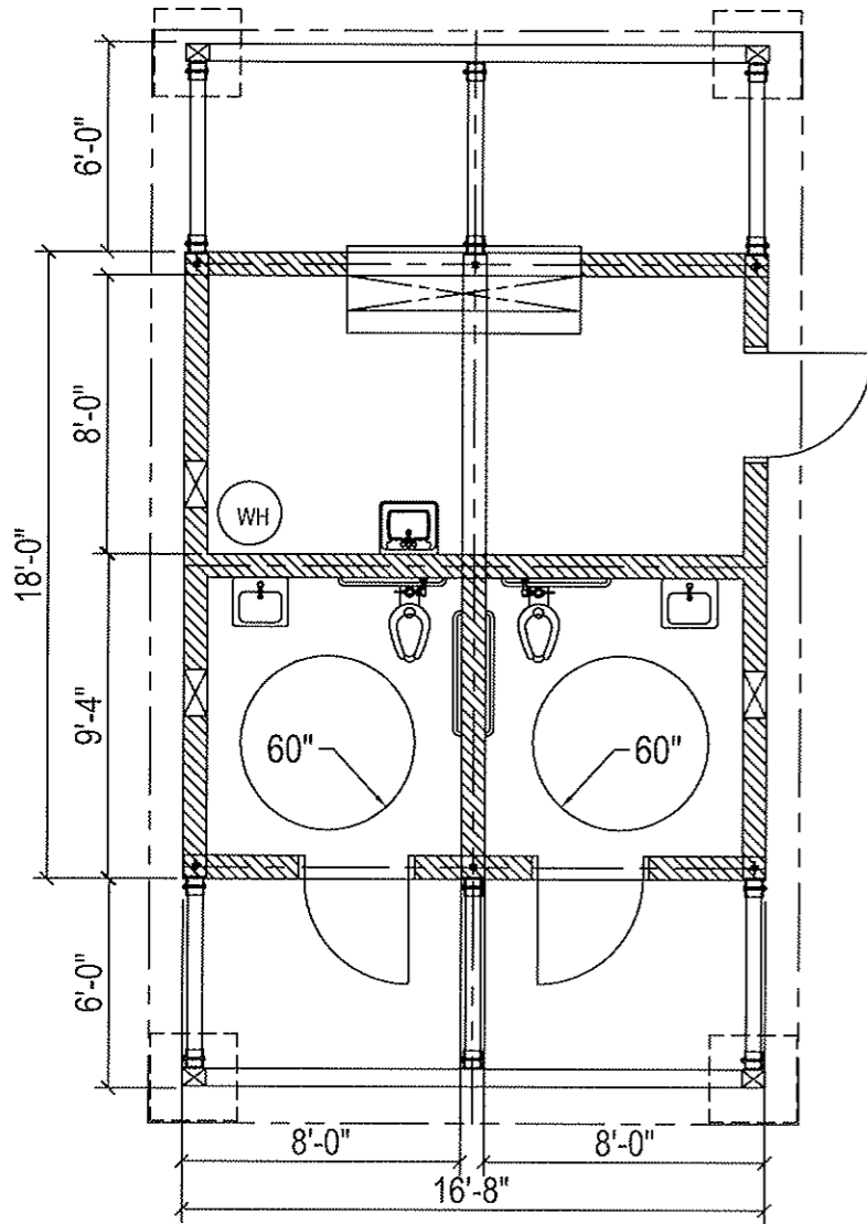
FLOOR PLAN
