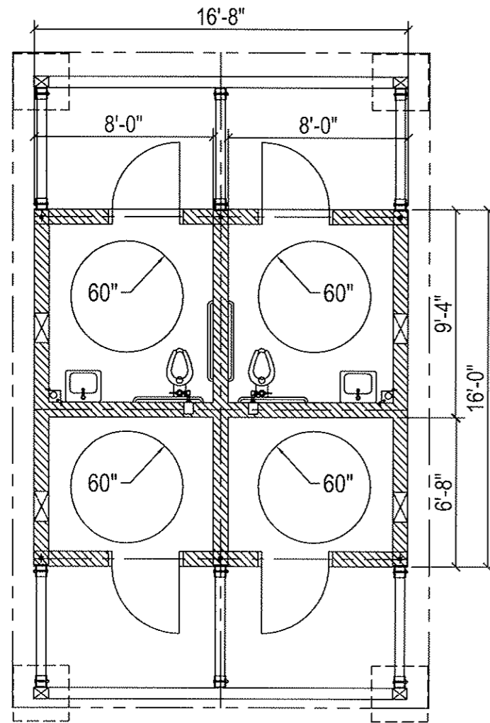
FLOOR PLAN
