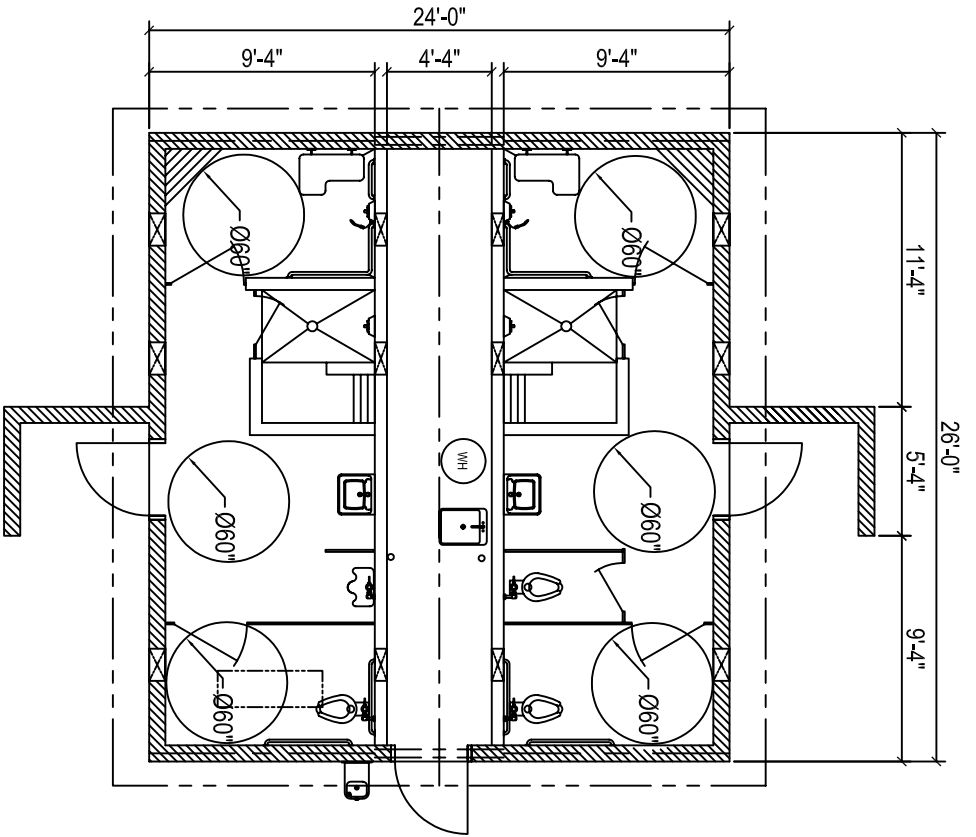
FLOOR PLAN
